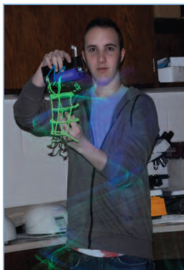
A model of green fluorescent protein.
